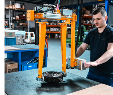
Battery gripper
