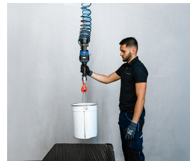
Bucket gripper
