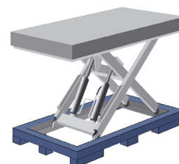
Fork lift entry base
